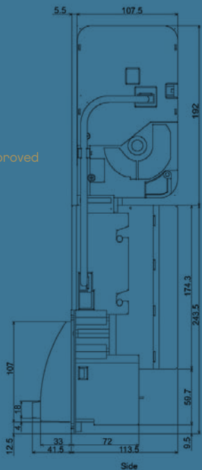
Side
